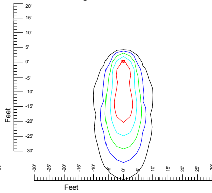
Mounting at 11'
