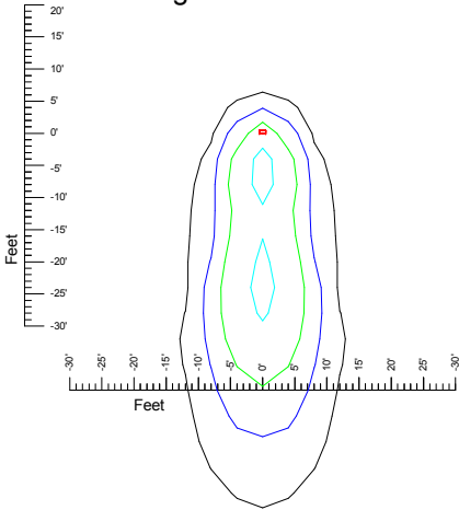
Mounting at 20'
