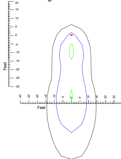
Mounting at 30'
