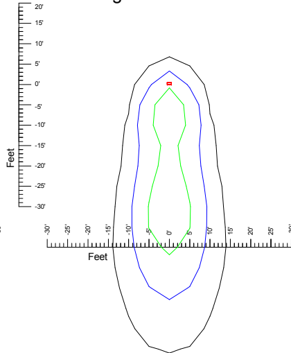
Mounting at 25'
