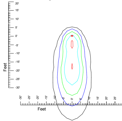
Mounting at 30'
