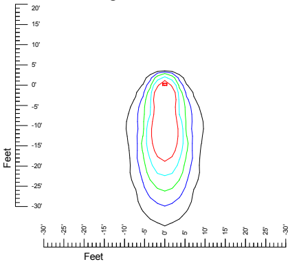
Mounting at 9'
