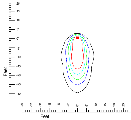
Mounting at 15'
